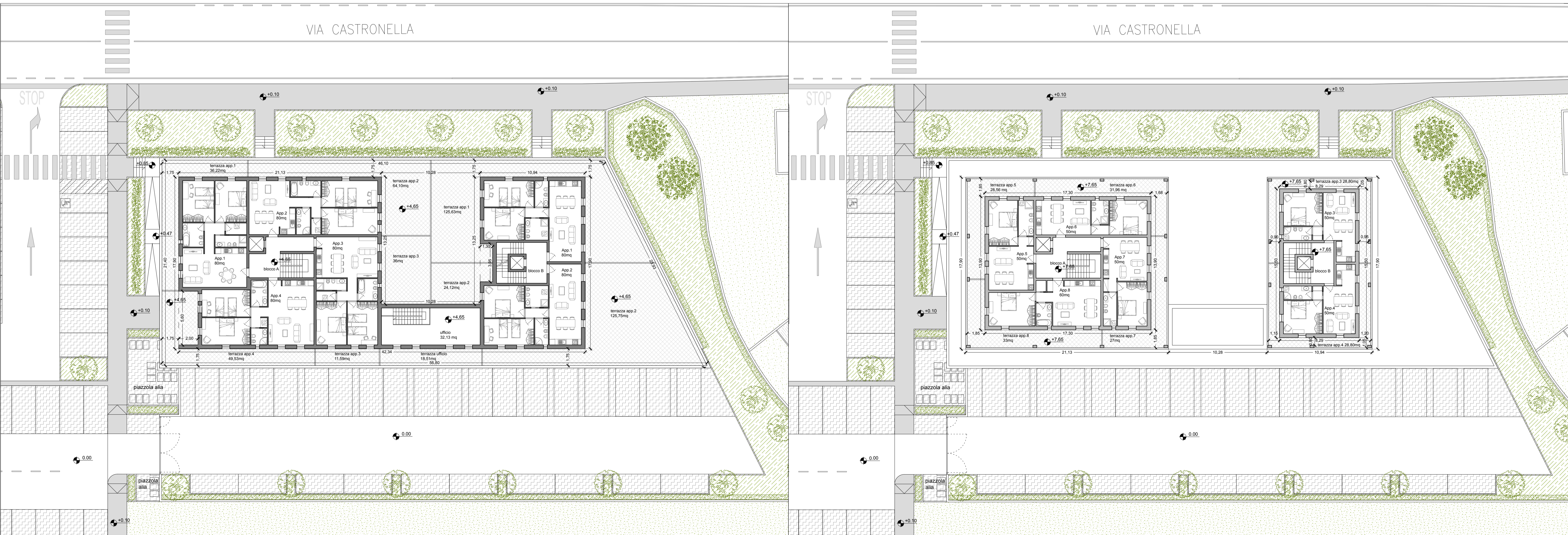
piano terra
